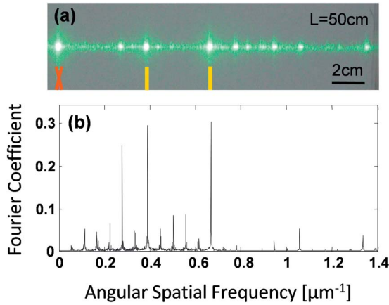
FIG. 1. (Color online) (a) The diffraction pattern photograph of the quasi-periodic nonlinear photonic crystal where the two relevant Fourier frequencies are marked. The dc component is marked with a red cross. (b) Fourier transform of the theoretical quasiperiodic design.
