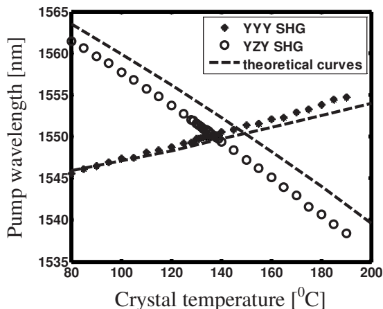
FIG. 2. Experimental results and theoretical curves of the two SHG interactions, showing the phase-matched wavelength dependence on temperature for the type I YYY and type II YZY processes. The intersection points of the measured and theoretical processes are different due to inaccuracies of the Sellmeier equation for ordinary polarization.
