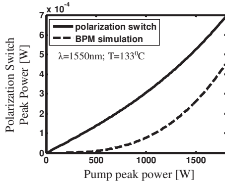
FIG. 4. The polarization switched peak power as a function of the pump peak power.
